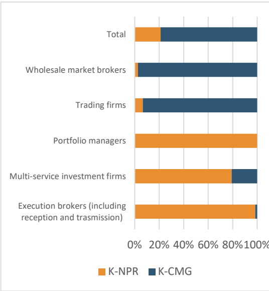
Figure 4 Marginal contribution of K-NPR and K-CMG to K-RtM
